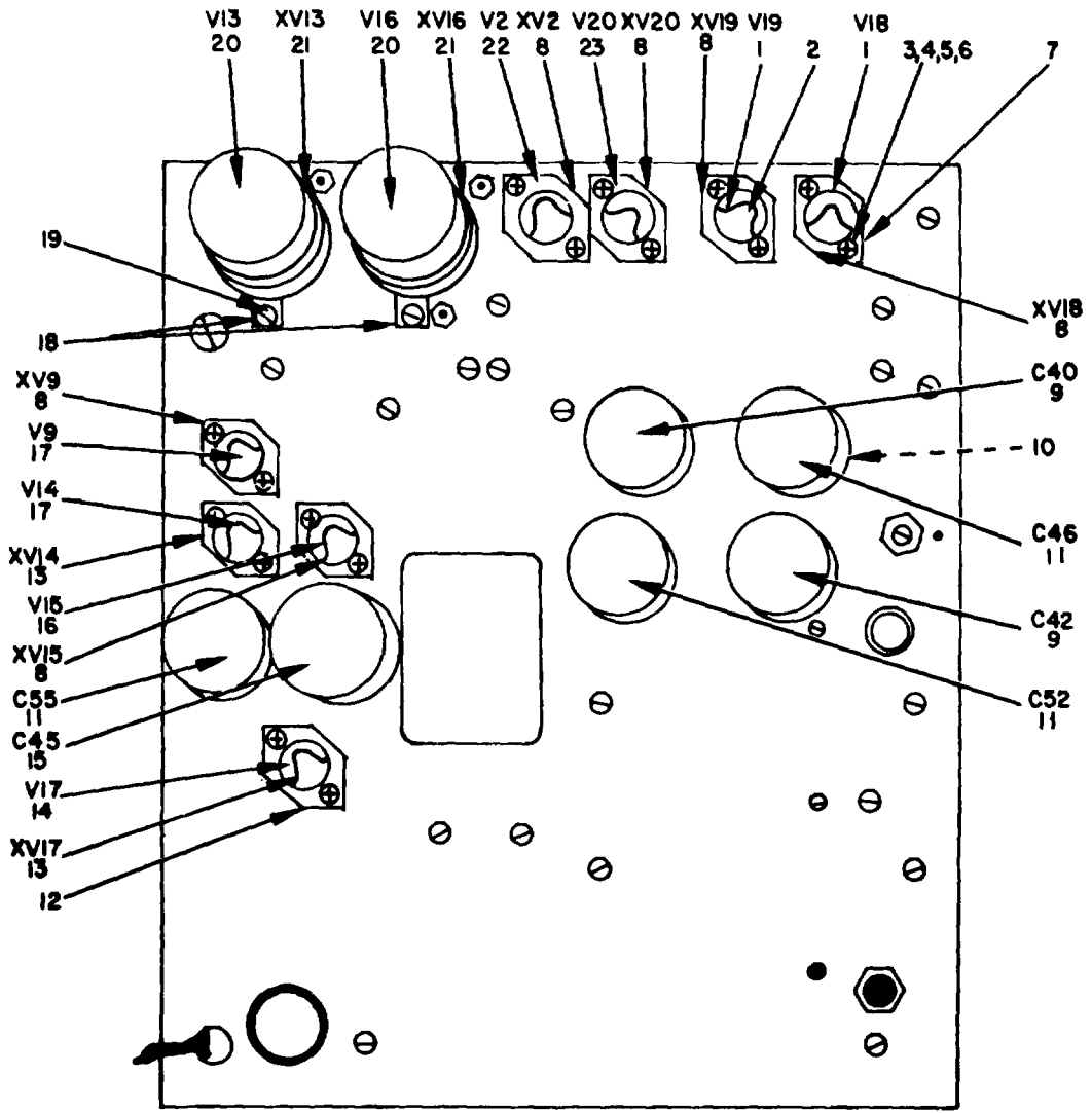
CHASSIS ASSEMBLY, TOP VIEW
